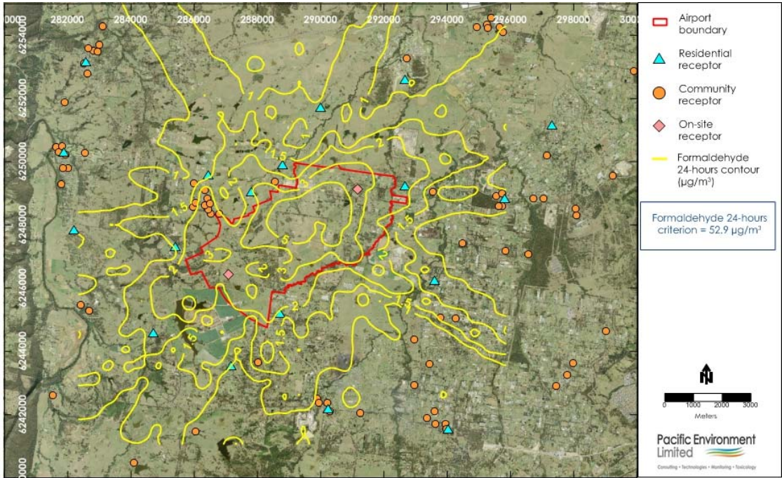
Figure F39: Formaldehyde 24-hour Contour Plot during Stage 1 development - Airport
