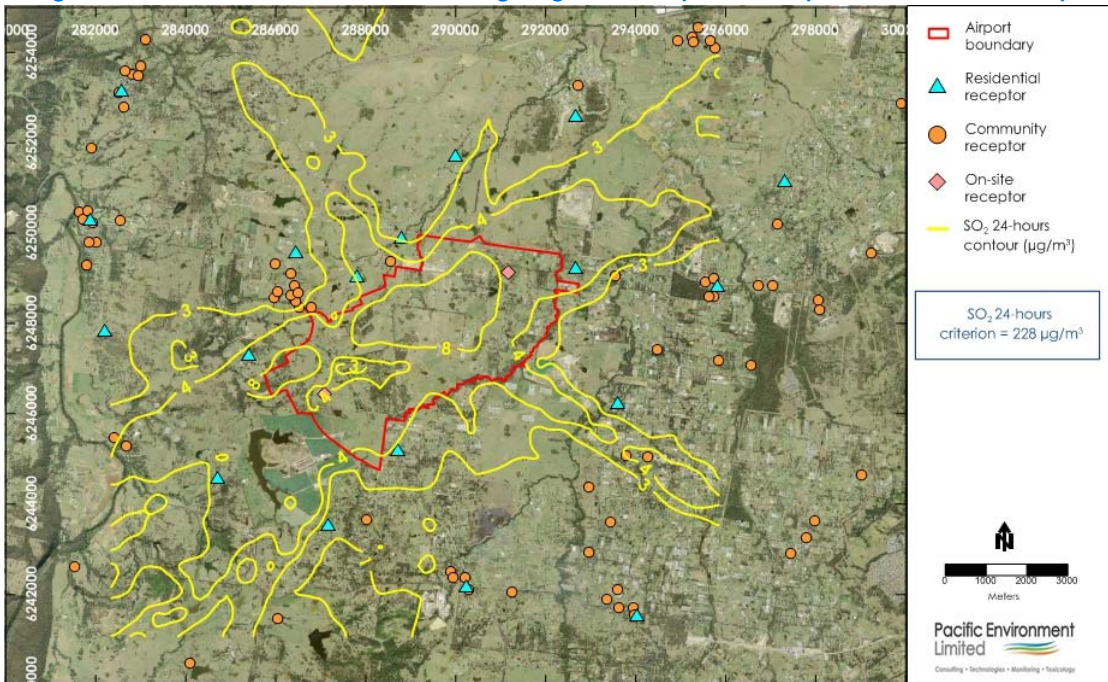
Figure F24: SO 2 24-hours Contour Plot during Stage 1 development – Airport + External Roadways
