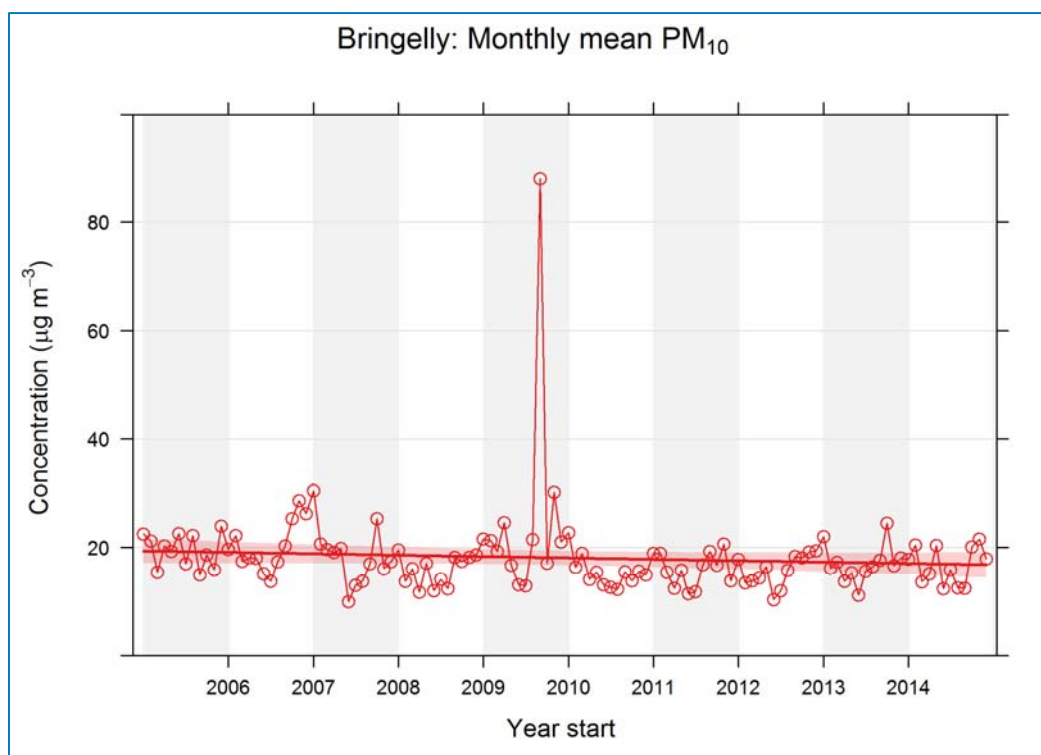
Figure 4-13: Monthly mean \text{PM}_{10} concentrations at Bringelly
