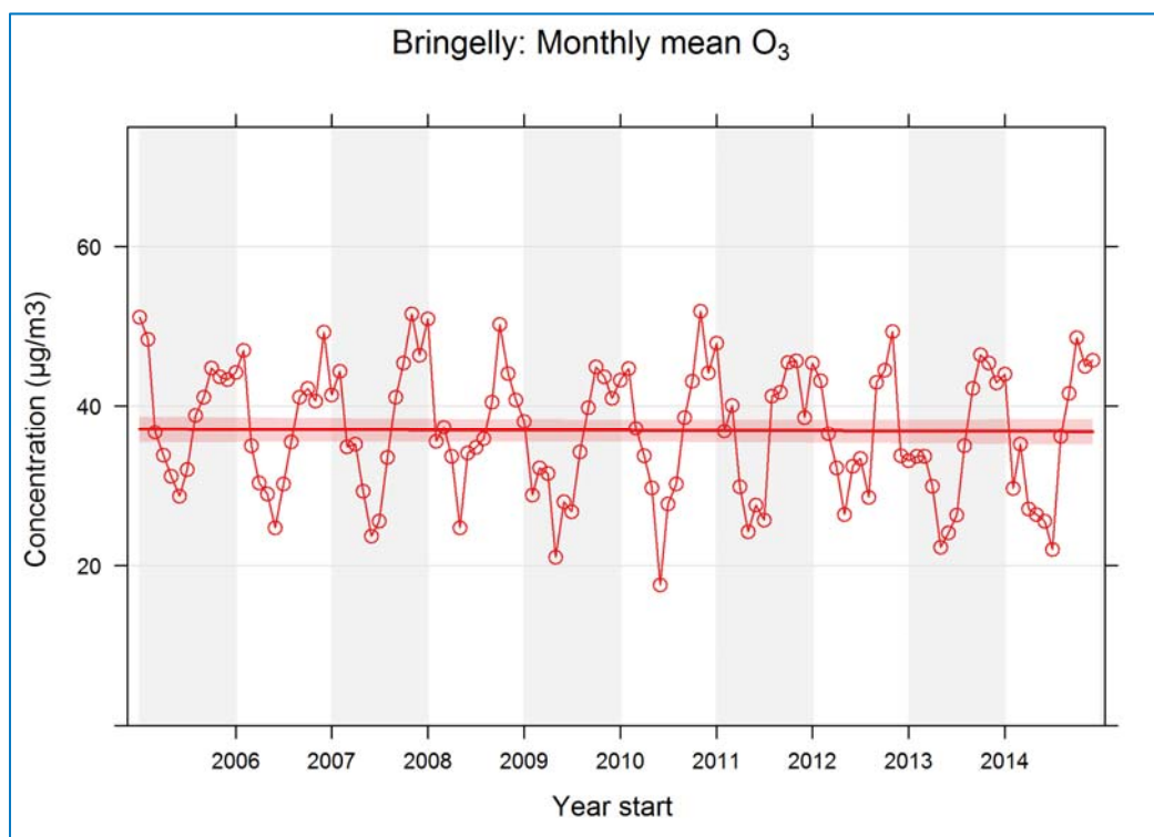
Figure 4-12: Monthly mean O 3 concentrations at Bringelly
