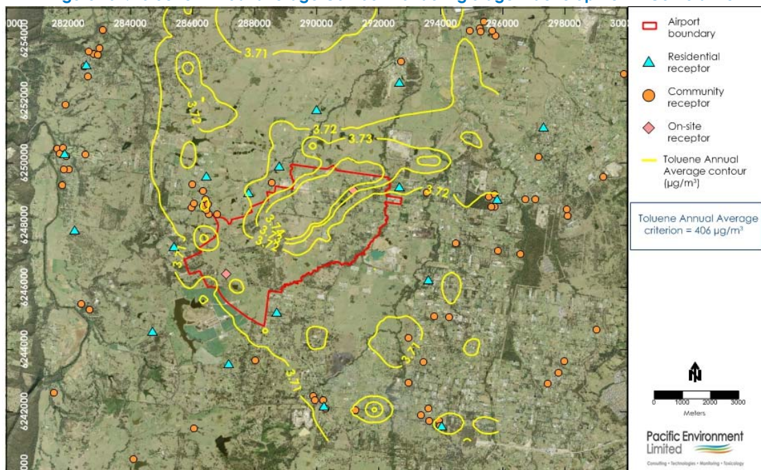
Figure F54: Toluene Annual average Contour Plot during Stage 1 development - Cumulative
