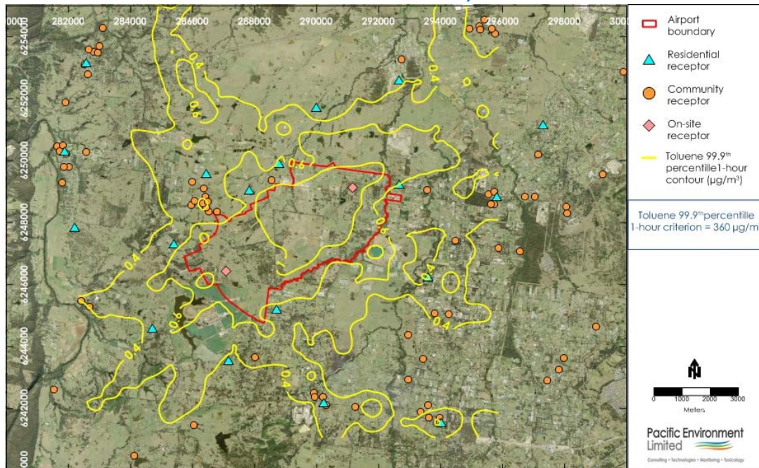
Figure F34: Toluene 99.9th percentile 1-hour average Contour Plot during Stage 1 development – Airport + External Roadways
