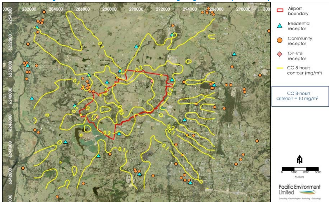
Figure F15: CO 8-hour Contour Plot during Stage 1 development - Airport
