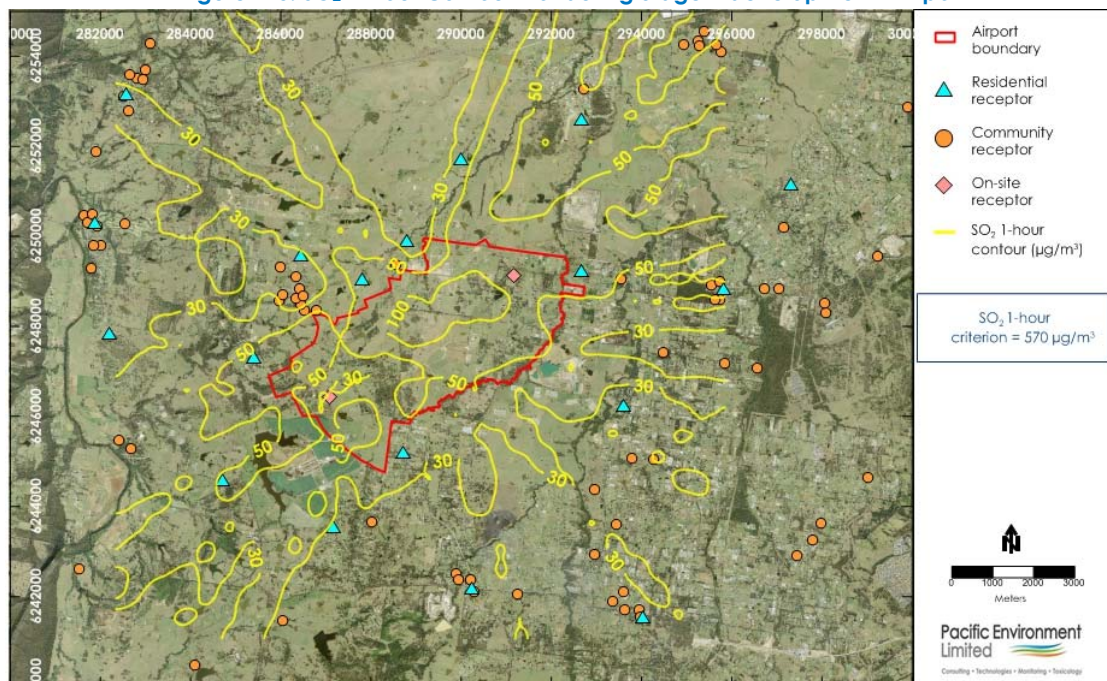
Figure F20: SO 2 1-hour Contour Plot during Stage 1 development –Airport
