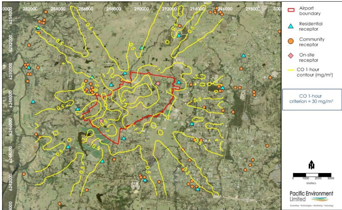
Figure F14: CO 1-hour Contour Plot during Stage 1 development - Airport
