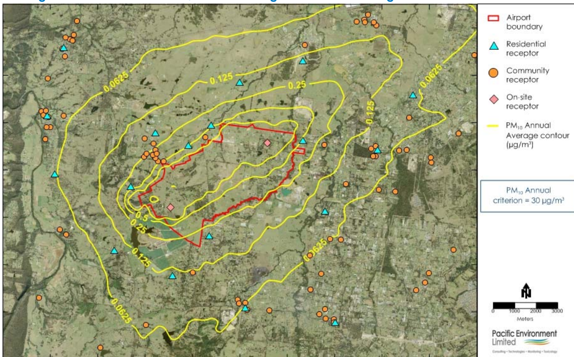
Figure G10: Incremental PM 10 Annual Average Contour Plot during aviation infrastructure works
