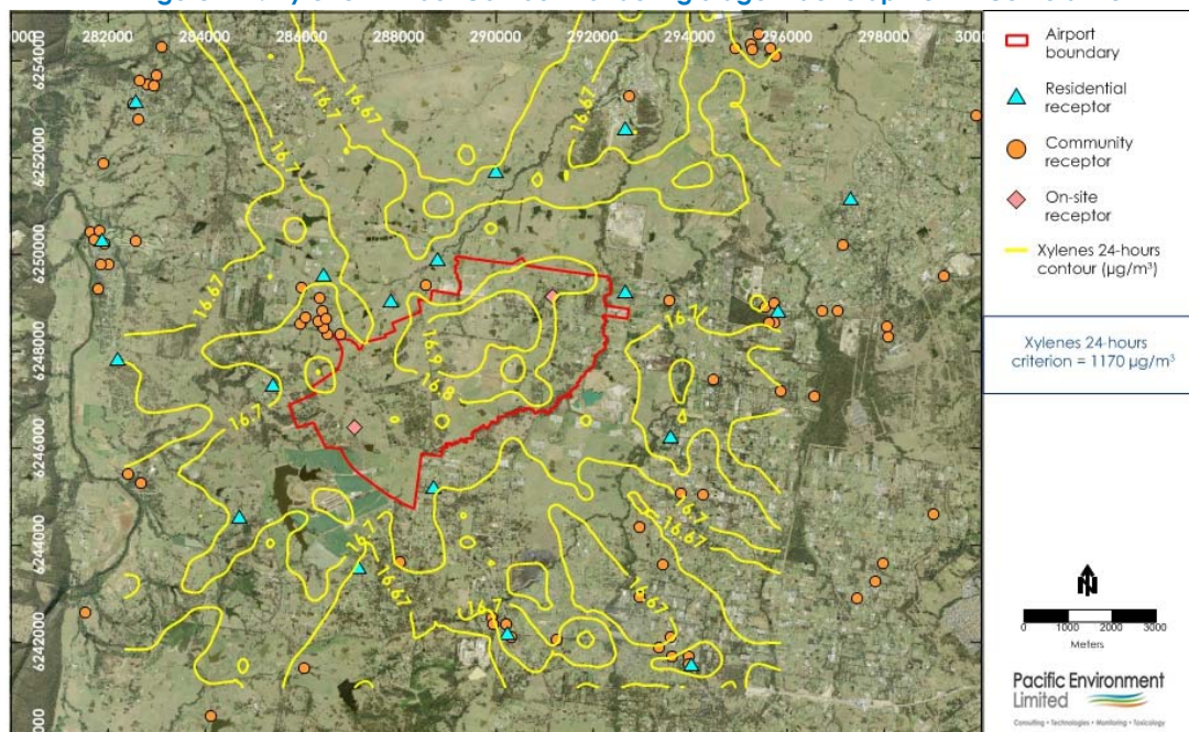
Figure F44: Xylene 24-hour Contour Plot during Stage 1 development – Cumulative
