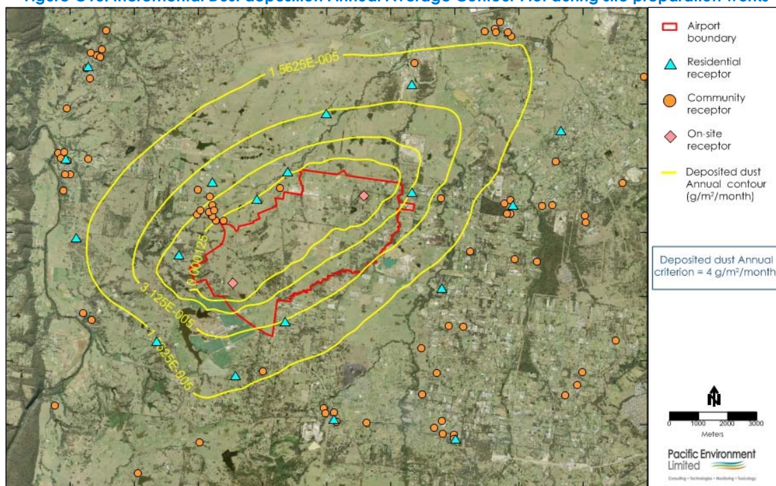
Figure G13: Incremental Dust deposition Annual Average Contour Plot during site preparation works
