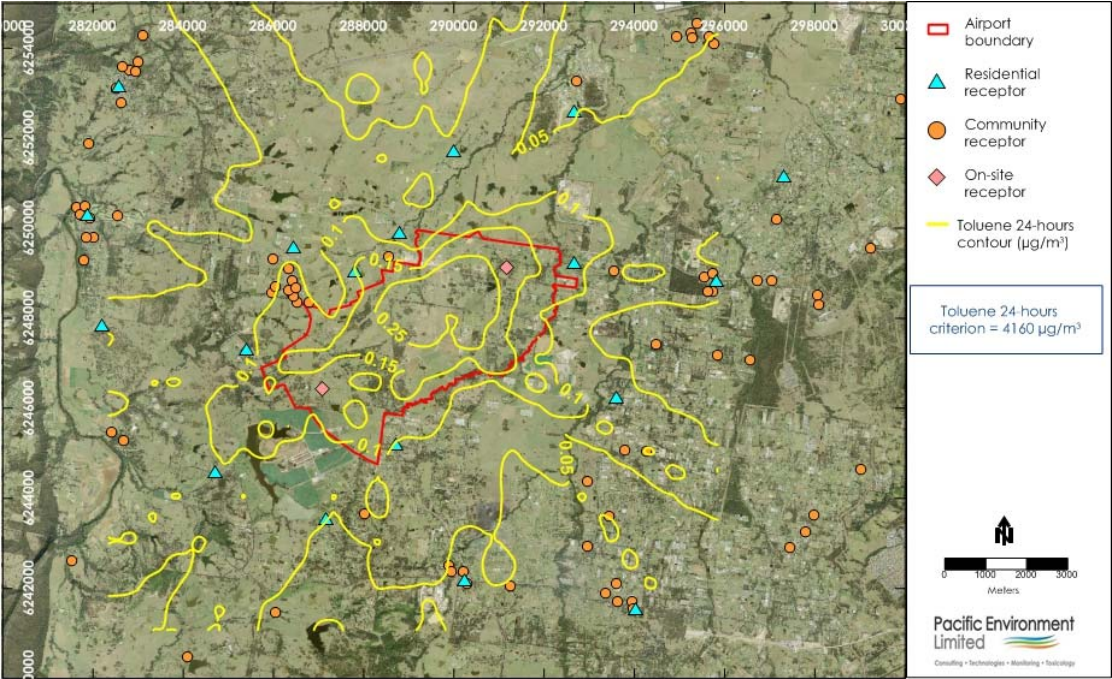
Figure F47: Toluene Annual average Contour Plot during Stage 1 development – Airport
