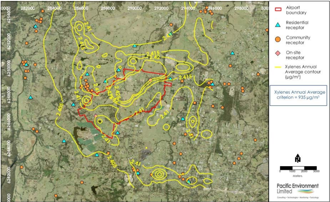
Figure F53: Xylene Annual average Contour Plot during Stage 1 development - Cumulative
