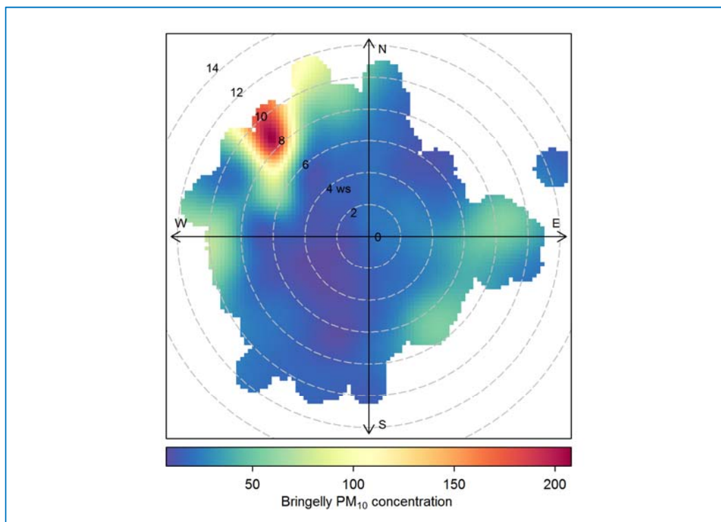
Figure 4-14: Polar plot of normalised PM 10 concentration at Bringelly
