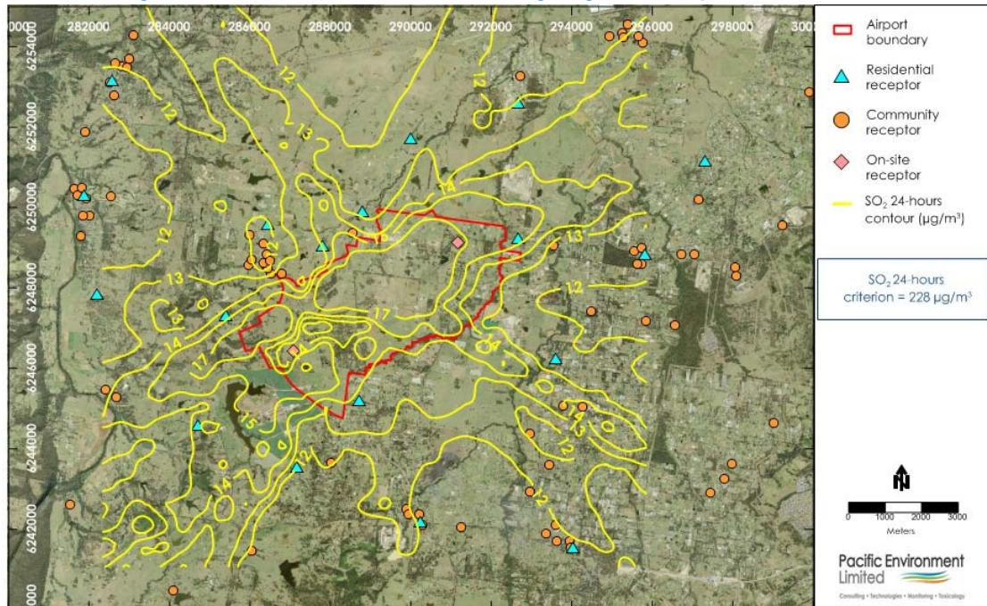
Figure F27: SO 2 24-hours Contour Plot during Stage 1 development - Cumulative
