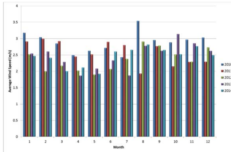
Figure 4-1 Monthly average wind speed at Badgerys Creek (2010-2014)
