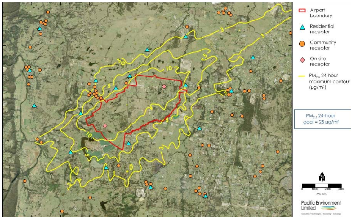
Figure G3: Incremental PM 2.5 24-hours Contour Plot bulk earthworks
