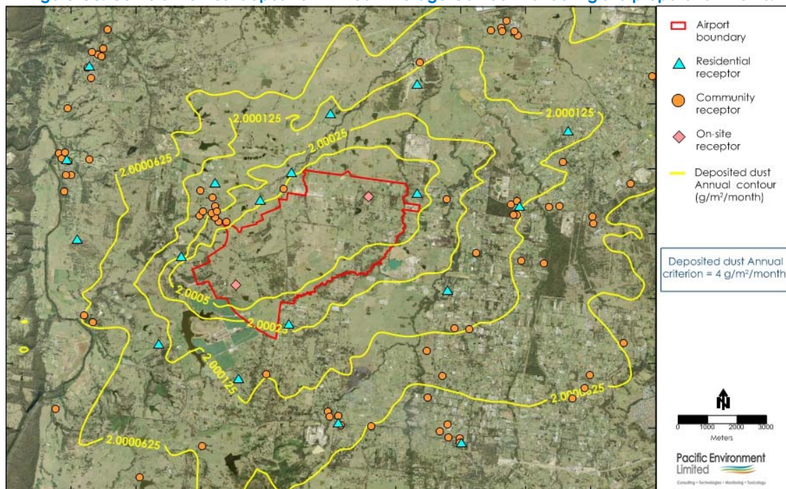
Figure G8: Cumulative Dust deposition Annual Average Contour Plot during site preparation works.
