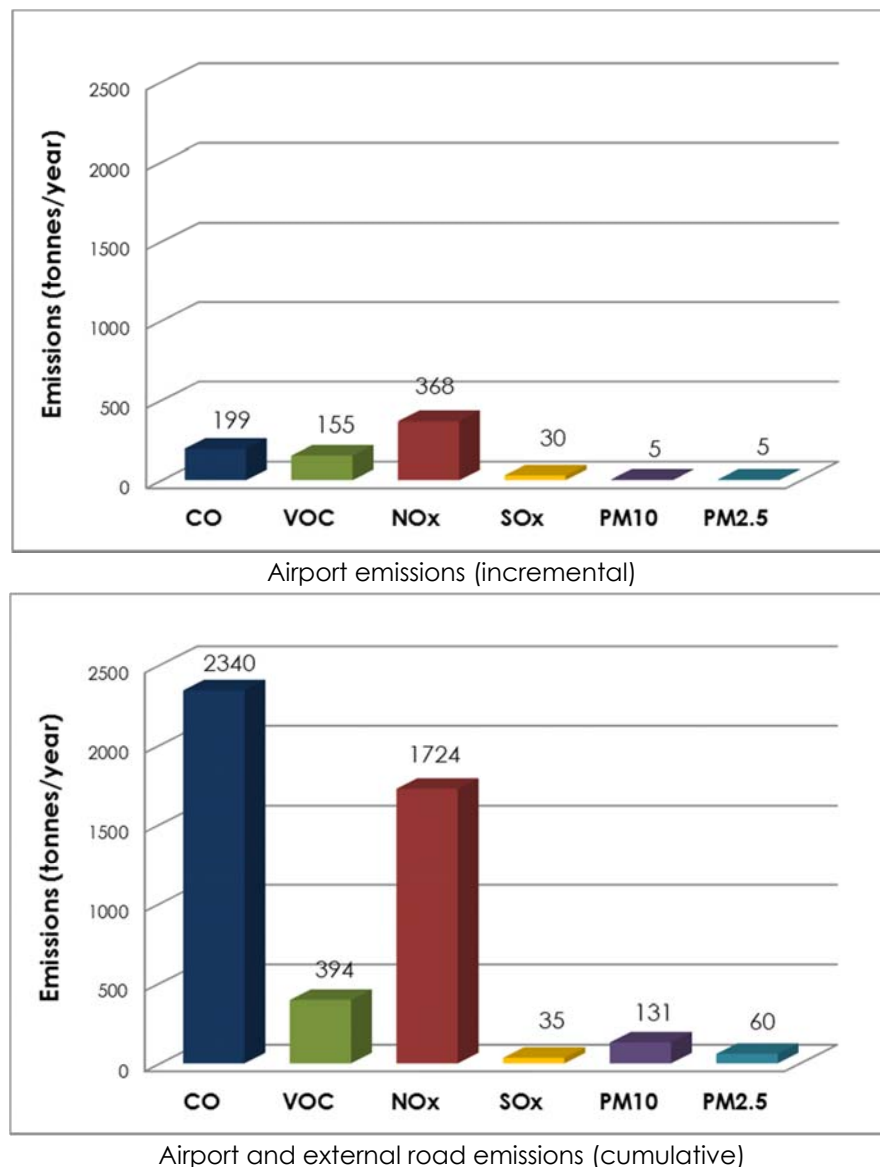
Figure 5-1: Total estimated emissions for criteria pollutants during Stage 1 development
