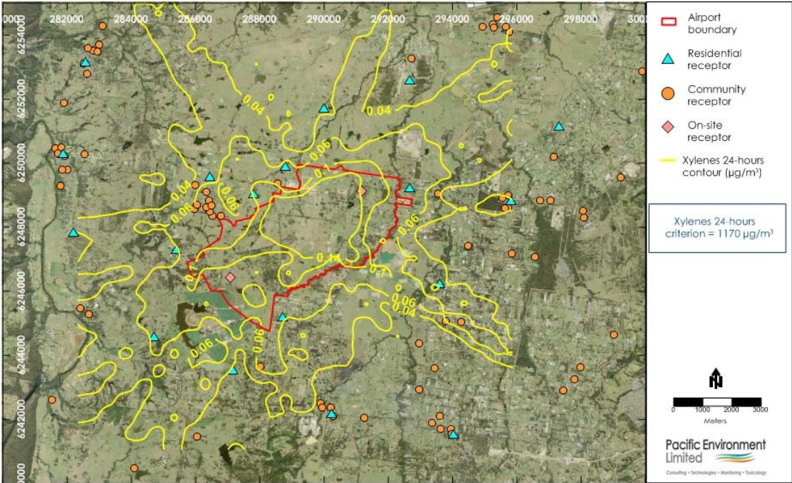
Figure F37: Xylene 24-hour Contour Plot during Stage 1 development – Airport
