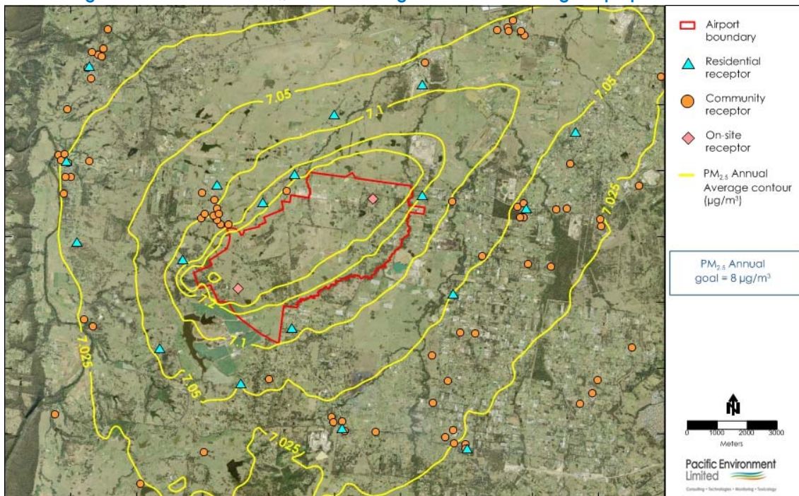
Figure G7: Cumulative PM 2.5 Annual Average Contour Plot during site preparation work
