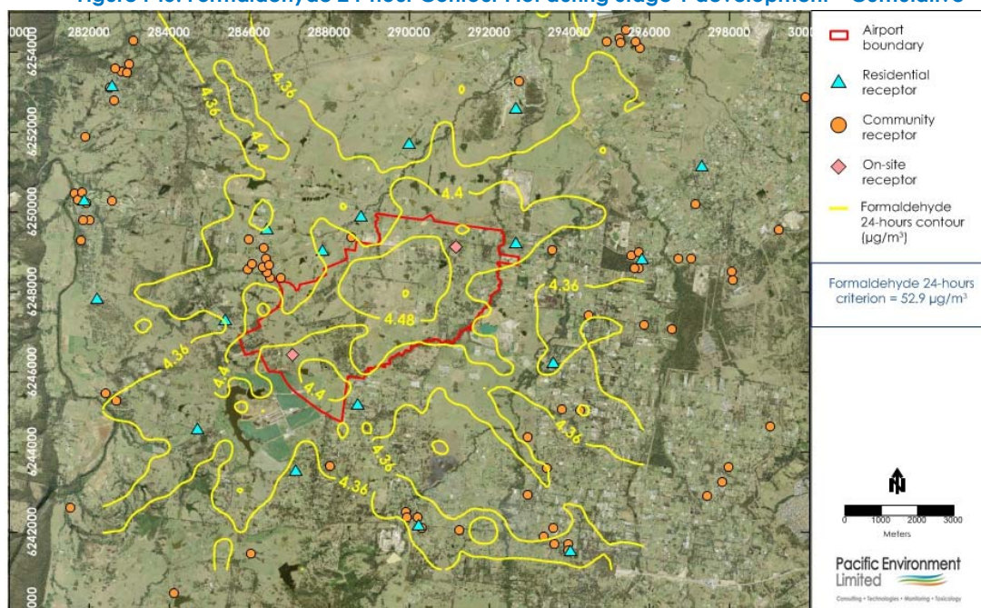
Figure F45: Formaldehyde 24-hour Contour Plot during Stage 1 development – Cumulative
