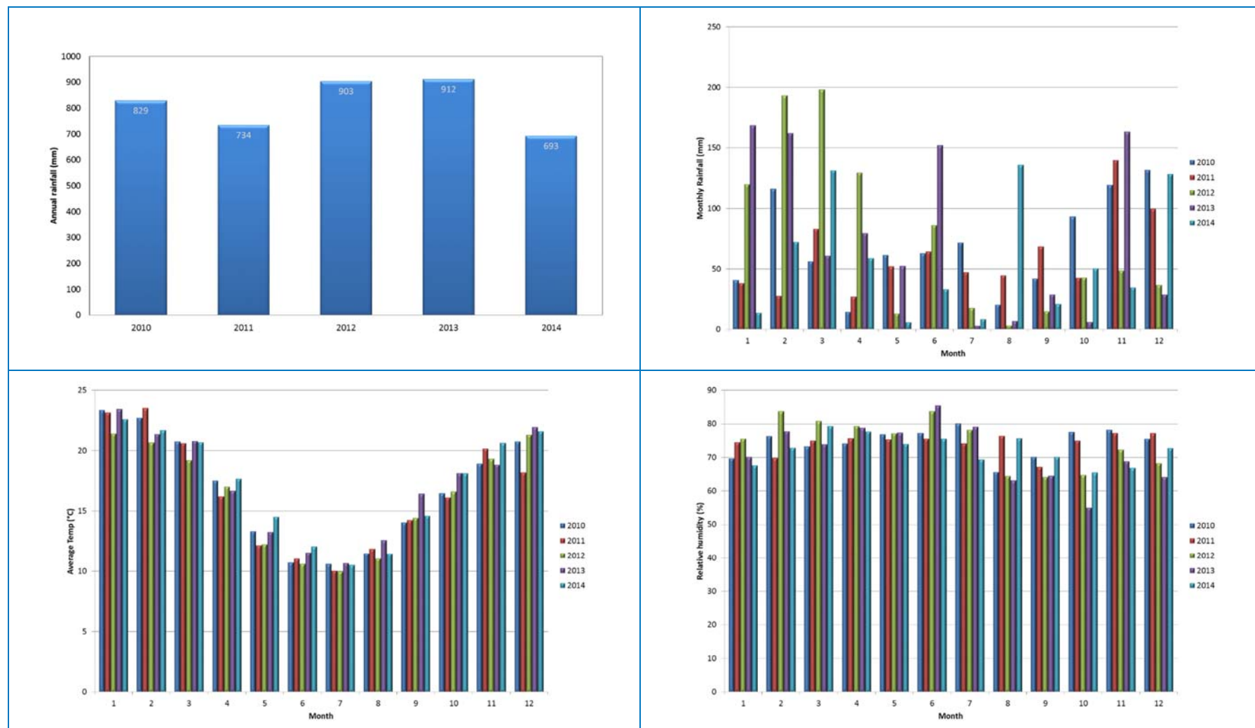
Figure 4-7 Annual and monthly average rainfall, temperature and relative humidity at Badgerys Creek (2010-2014)
