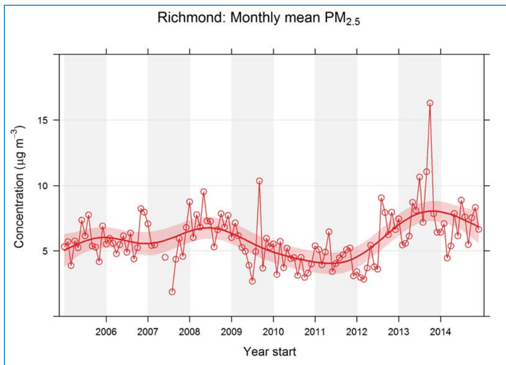
Figure 4-16: Monthly mean PM 2.5 concentrations at Richmond
