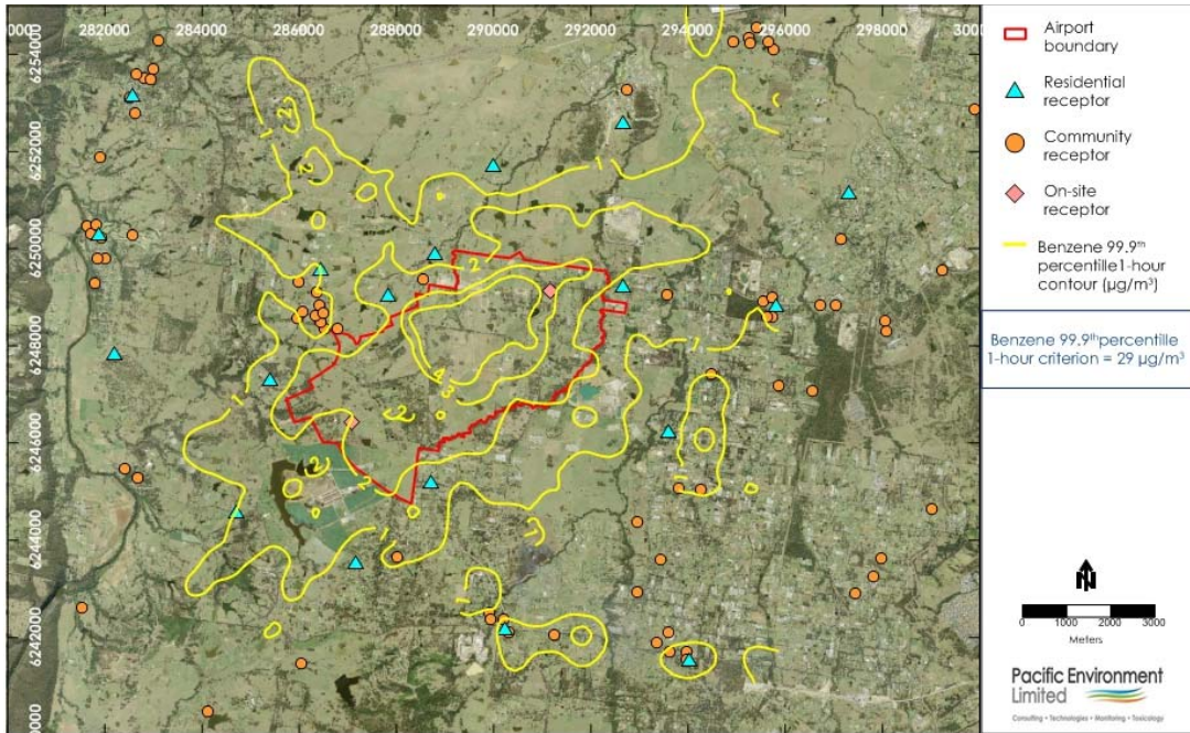
Figure F33: Benzene 99.9th percentile 1-hour average Contour Plot during Stage 1 development – Airport + External Roadways
