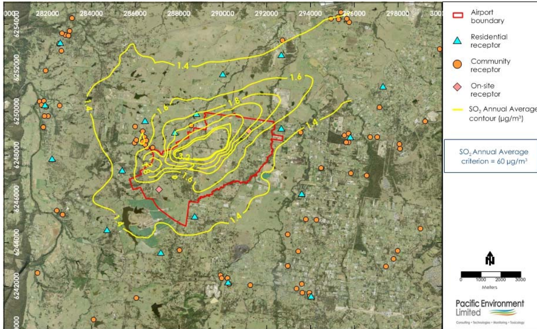
Figure F28: SO 2 Annual Average Contour Plot during Stage 1 development - Cumulative.
