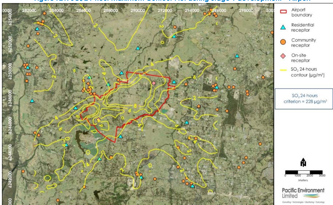
Figure F21: SO 2 24-hour Maximum Contour Plot during Stage 1 development – Airport
