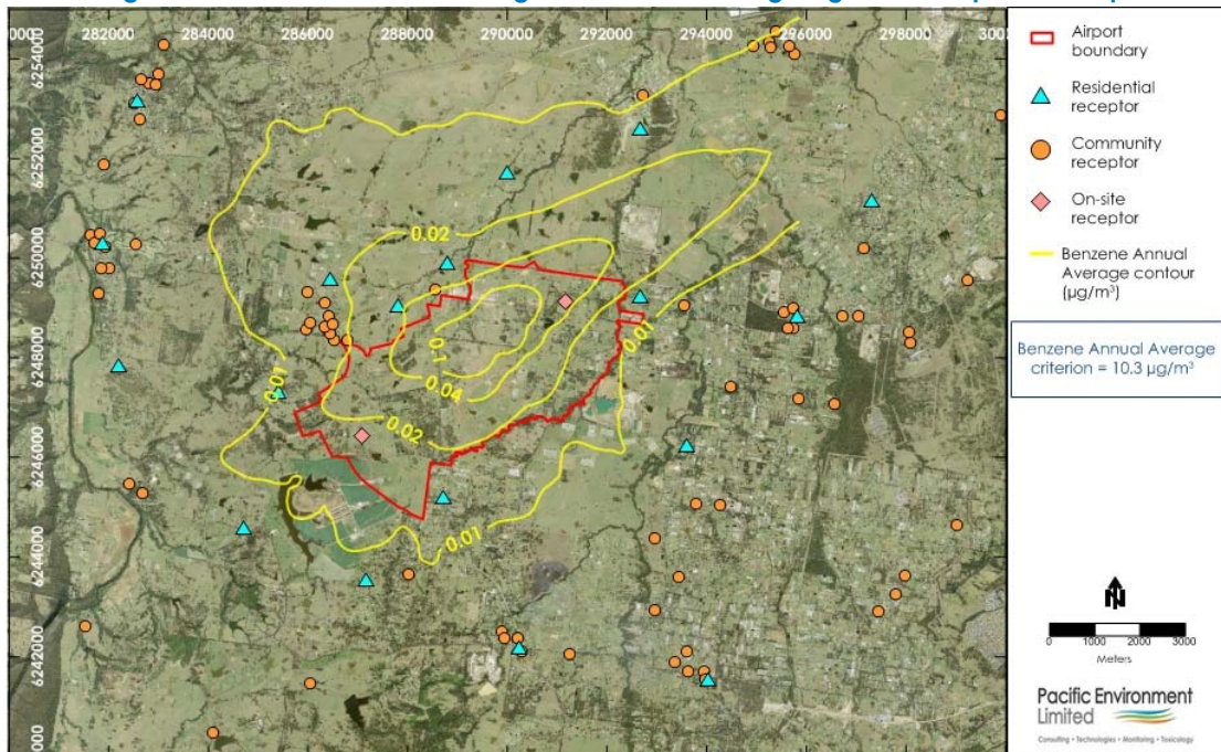
Figure F46: Benzene Annual average Contour Plot during Stage 1 development – Airport
