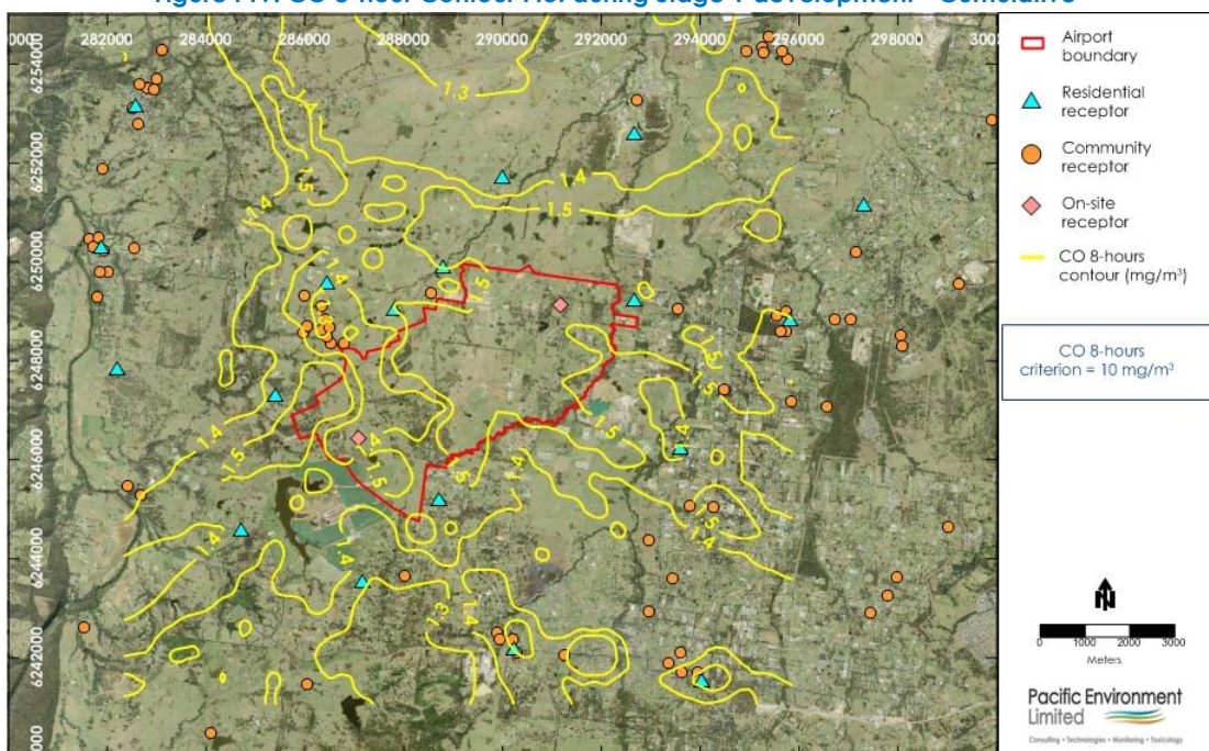
Figure F19: CO 8-hour Contour Plot during Stage 1 development - Cumulative
