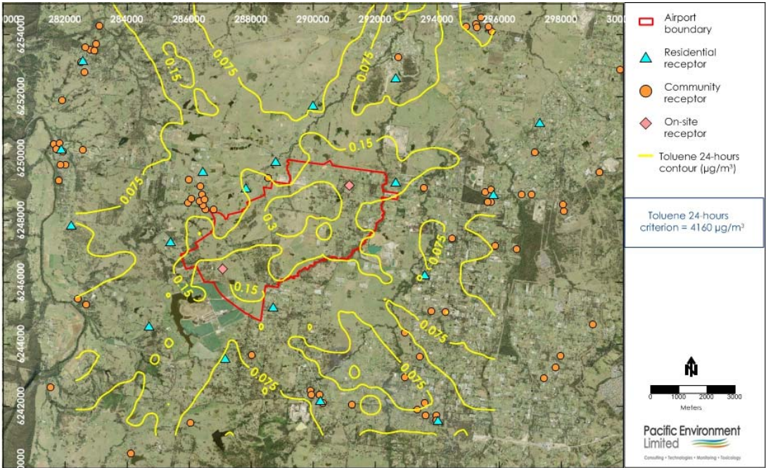
Figure F42: Toluene 24-hour Contour Plot during Stage 1 development – Airport + External Roadways
