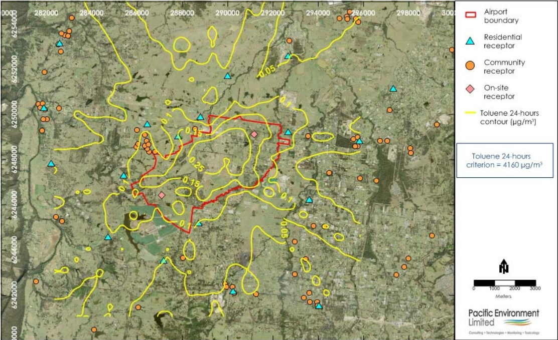
Figure F38: Toluene 24-hour Contour Plot during Stage 1 development – Airport
