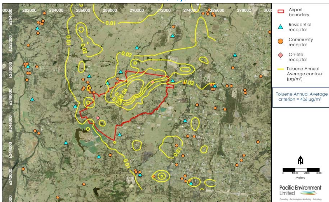
Figure F51: Toluene Annual average Contour Plot during Stage 1 development - Airport + External Roadways
