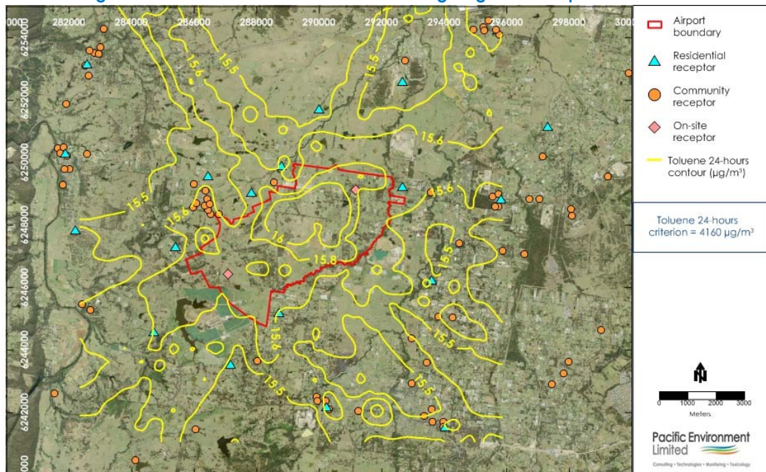
Figure F43: Toluene 24-hour Contour Plot during Stage 1 development – Cumulative
