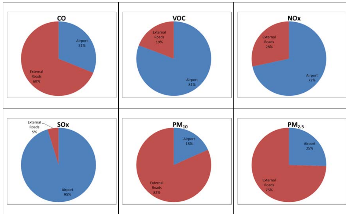
Figure 5-5: Estimated airport and external roads emissions as a percentage of total modelled for criteria pollutants during longer term development
