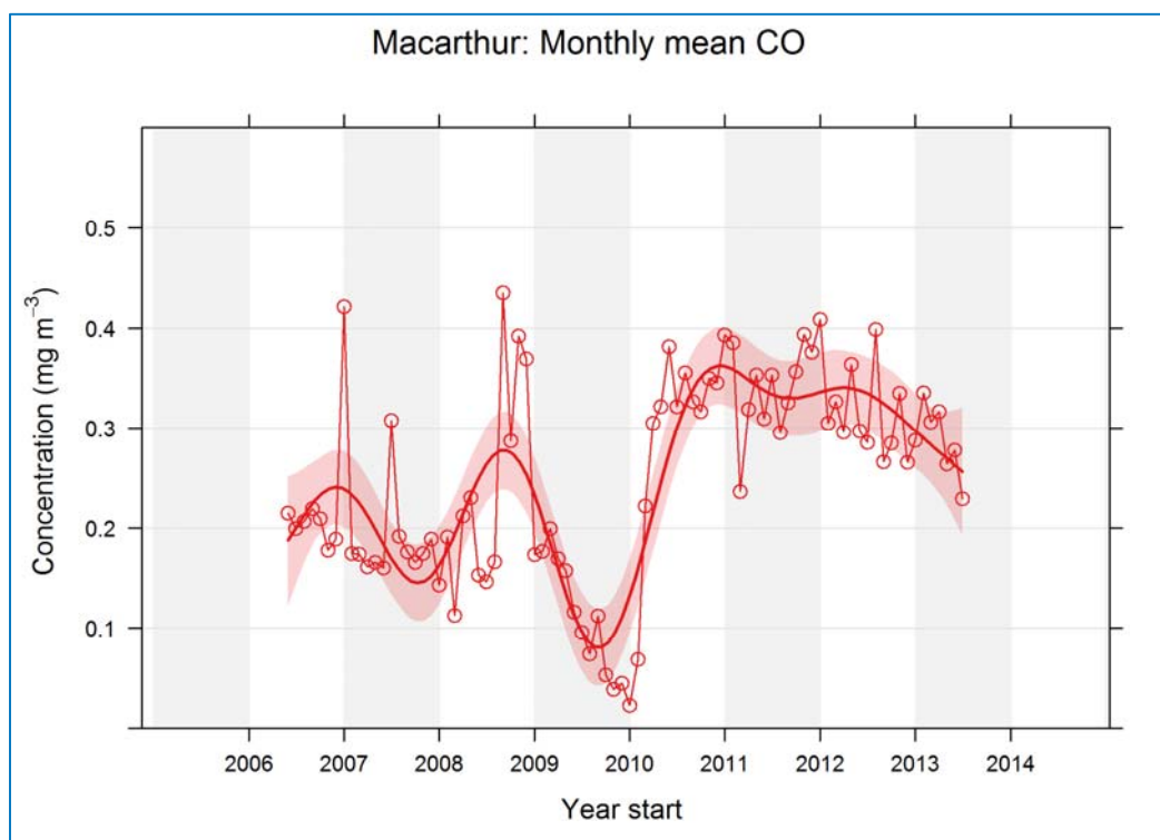
Figure 4-17: Monthly mean CO concentrations at Macarthur
