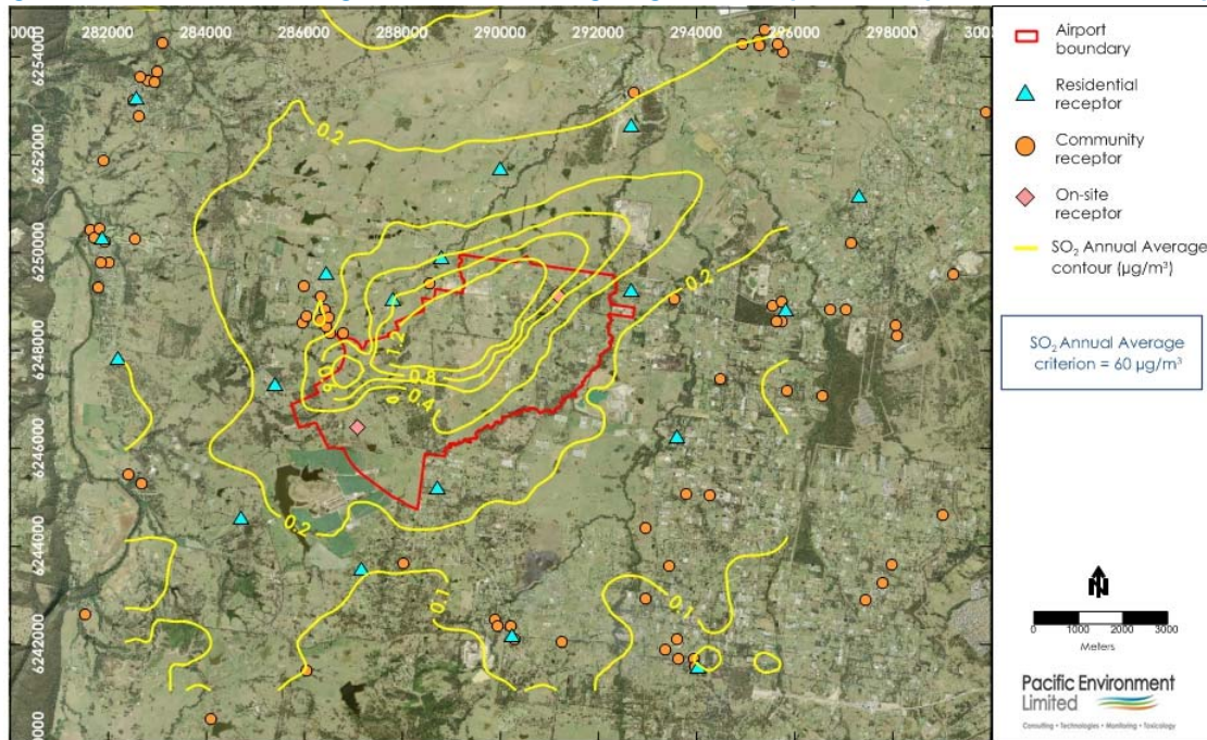
Figure F25: SO 2 Annual Average Contour Plot during Stage 1 development – Airport + External Roadways
