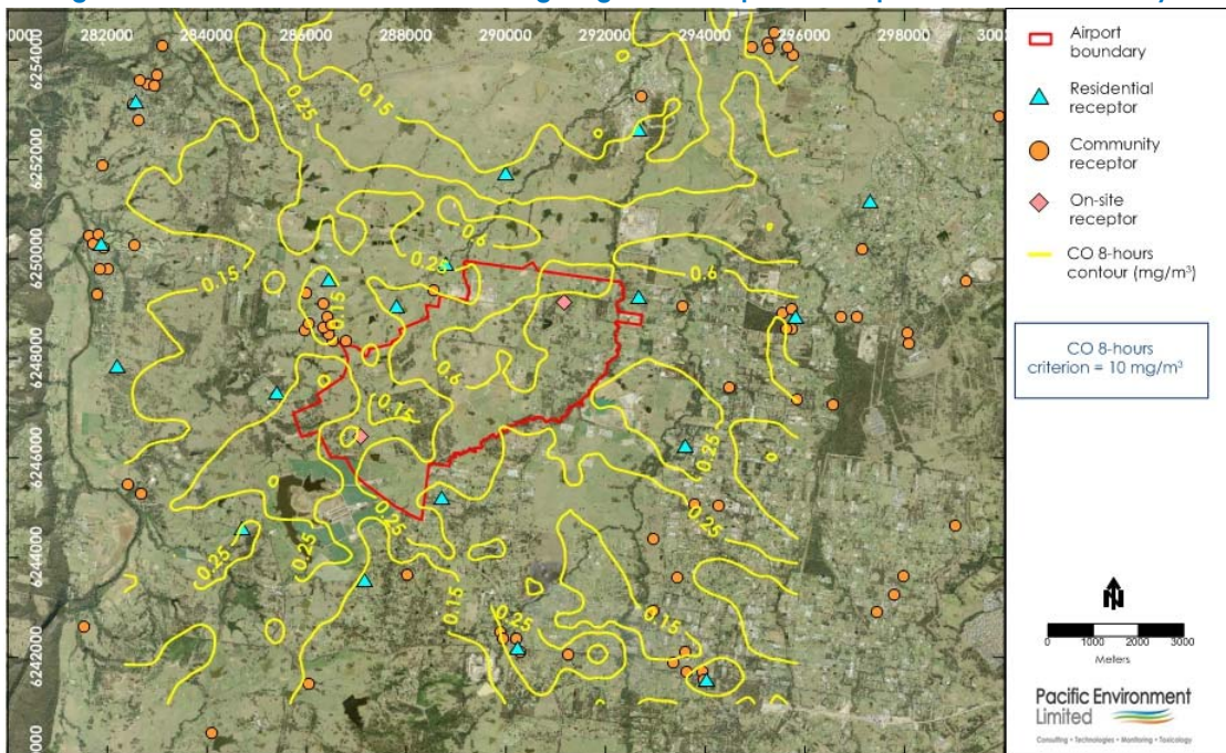
Figure F17: CO 8-hour Contour Plot during Stage 1 development - Airport + External Roadways
