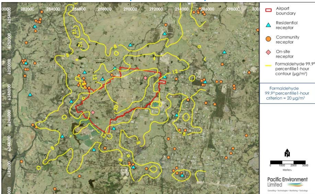
Figure F36: Formaldehyde 99.9th percentile 1-hour average Contour Plot during Stage 1 development – Airport + External Roadways
