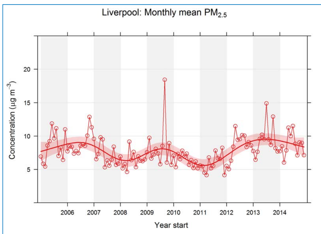
Figure 4-15: Monthly mean PM 2.5 concentrations at Liverpool
