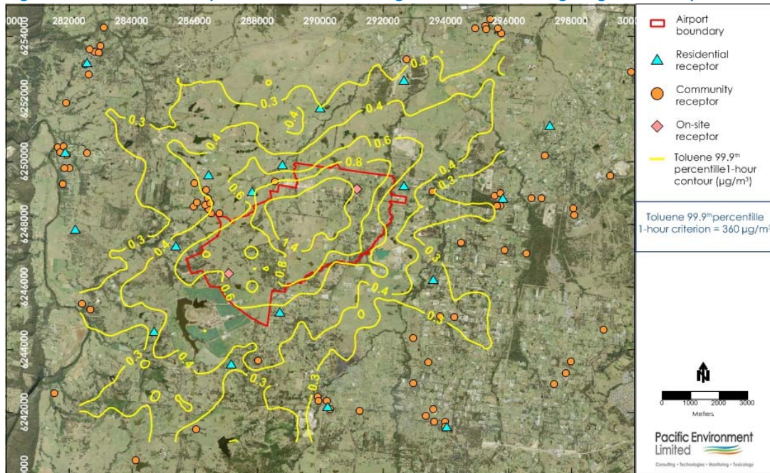
Figure F30: Toluene 99.9th percentile 1-hour average Contour Plot during Stage 1 development – Airport
