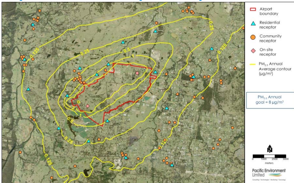
Figure G12: Incremental PM 2.5 Annual Average Contour Plot during aviation infrastructure works
