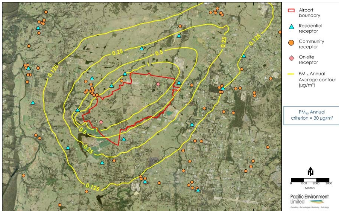
Figure G2: Incremental PM 10 Annual Average Contour Plot during bulk earthworks
