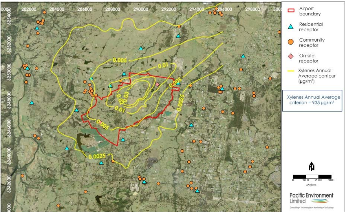
Figure F48: Xylene Annual average Contour Plot during Stage 1 development – Airport
