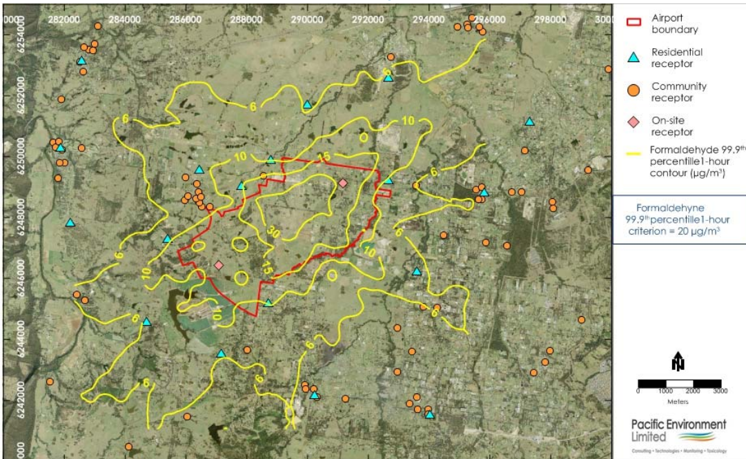
Figure F32: Formaldehyde 99.9th percentile 1-hour average Contour Plot during Stage 1 development – Airport
