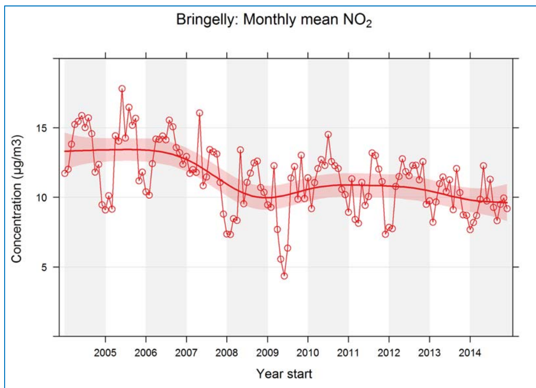
Figure 4-10: Monthly mean NO 2 concentrations at Bringelly
