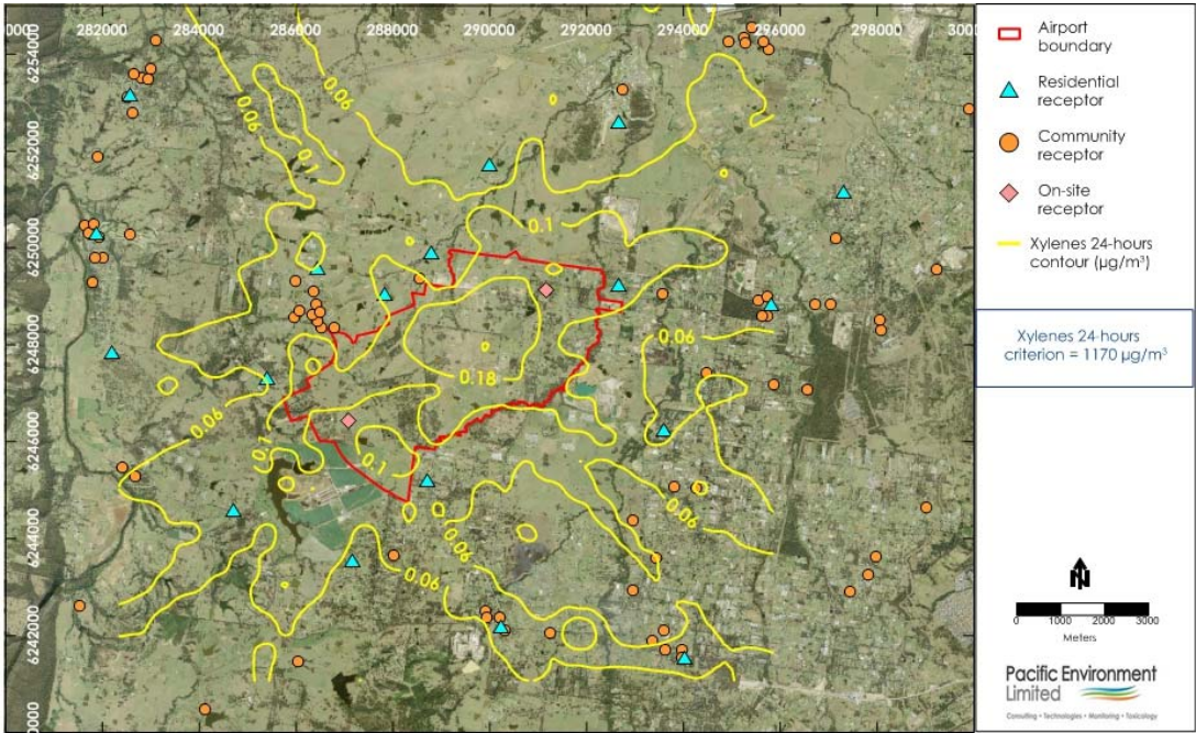
Figure F41: Xylene 24-hour Contour Plot during Stage 1 development – Airport + External Roadways
