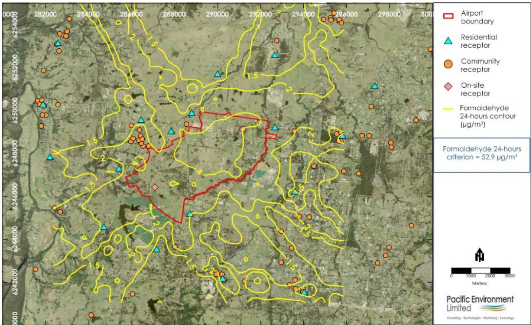
Figure F43: Formaldehyde 24-hour Contour Plot during Stage 1 development – Airport + External Roadways
