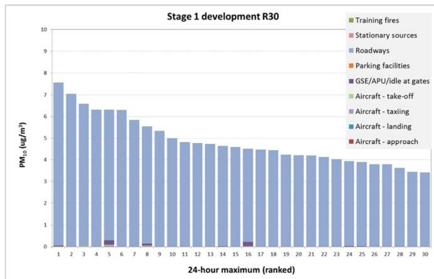
Figure 5-6: Contributions to PM 10 concentrations at R30
