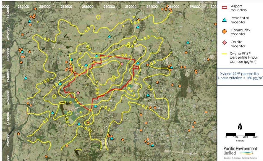
Figure F31: Xylene 99.9th percentile 1-hour average Contour Plot during Stage 1 development – Airport
