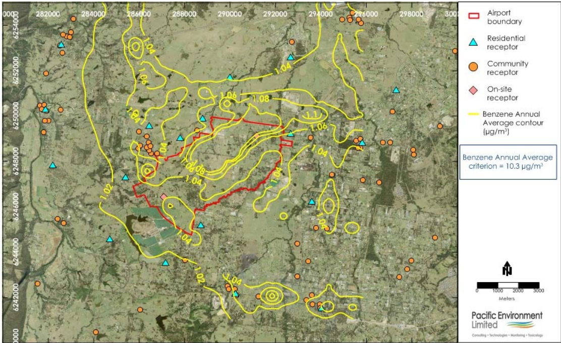
Figure F52: Benzene Annual average Contour Plot during Stage 1 development - Cumulative.
