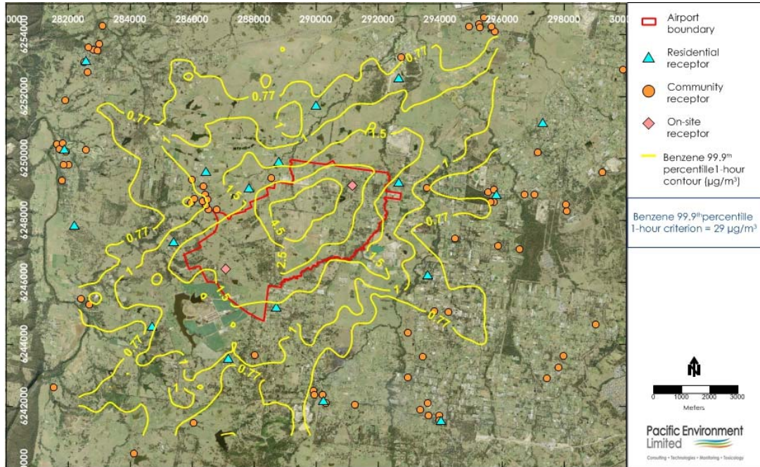
Figure F29: Benzene 99.9th percentile 1-hour average Contour Plot during Stage 1 development – Airport
