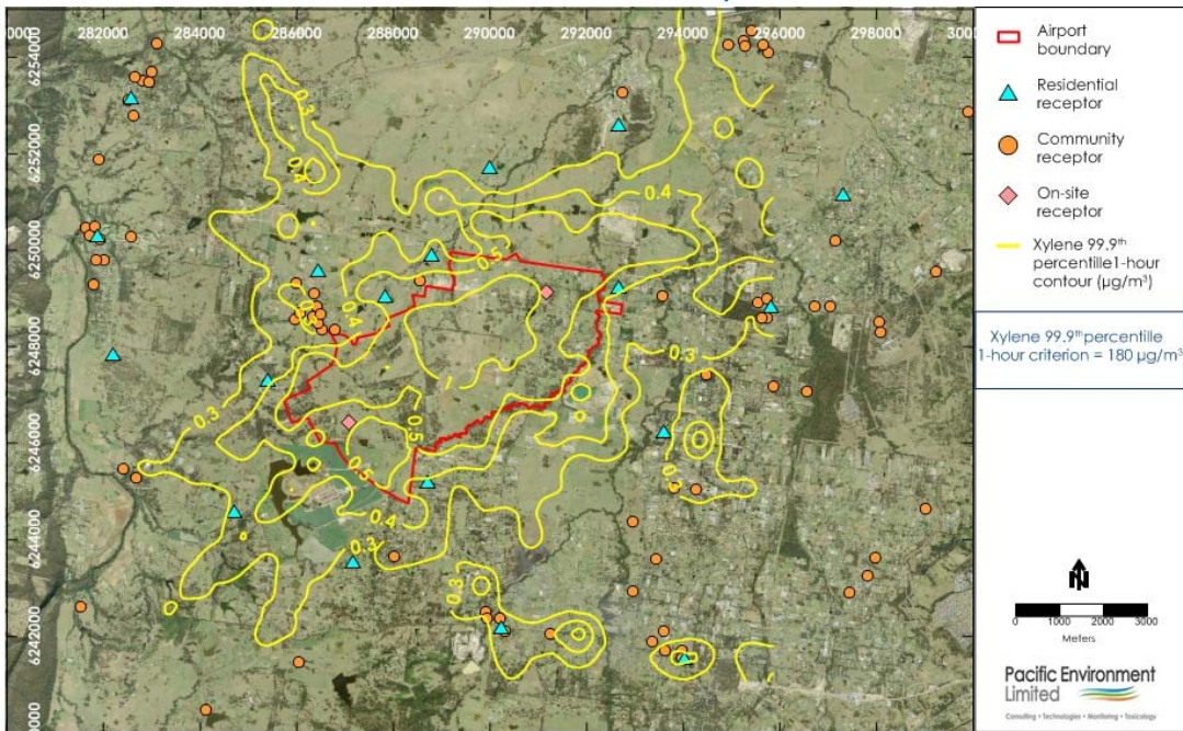
Figure F35: Xylene 99.9th percentile 1-hour average Contour Plot during Stage 1 development – Airport + External Roadways
