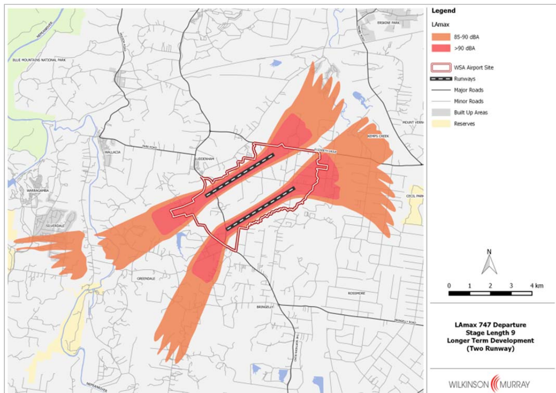
Figure 6-3 85 dBA & 90 dBA L_{Amax} Contours – B747 Departure – Longer Term Airport Development
