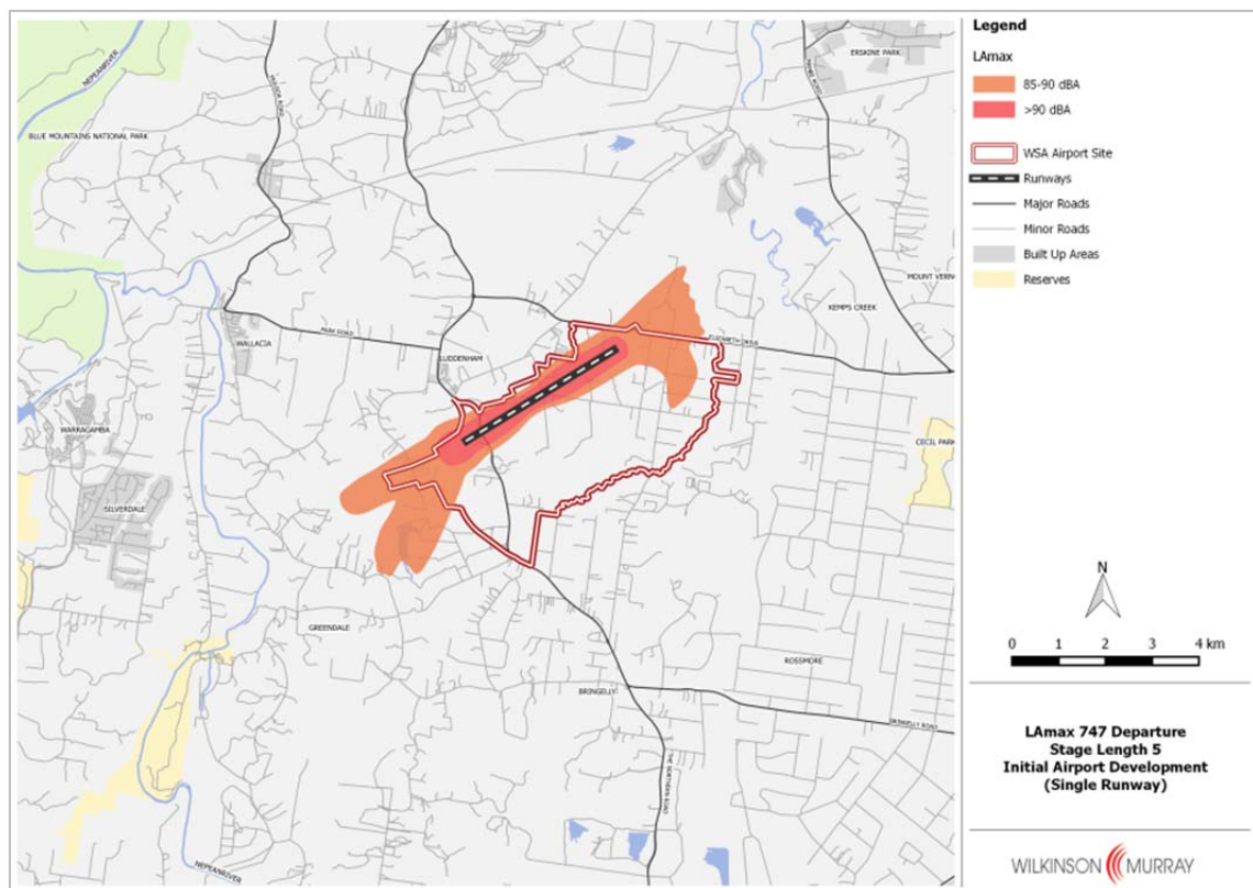
Figure 6-1 85 dBA & 90 dBA L_{Amax} Contours – B747 Departure Stage 5 – Initial Airport Development
