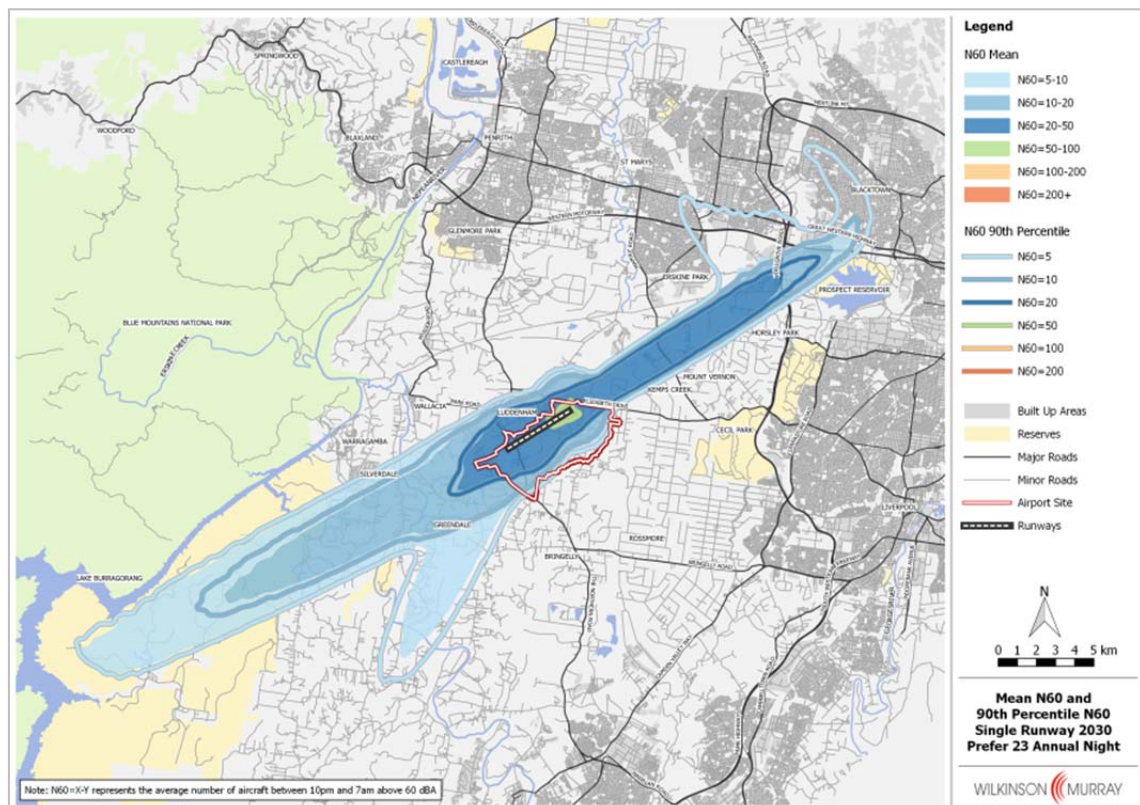
Figure 3-22 Mean & 90 th Percentile N60 Contours – 2030 – Prefer 23
